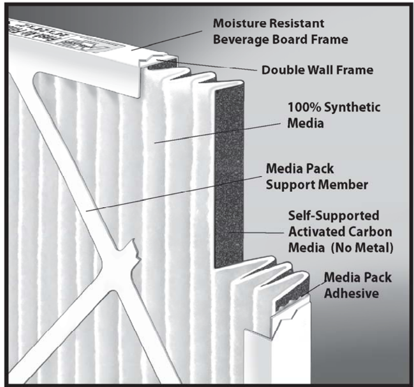
Increased carbon loading – now contains 200 grams per square meter of 60% activity carbon. Electrostatically charged media provides a MERV-7 performance.
